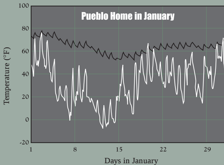
Time/temperature performance of the Pueblo home with the heating system turned off during January.
