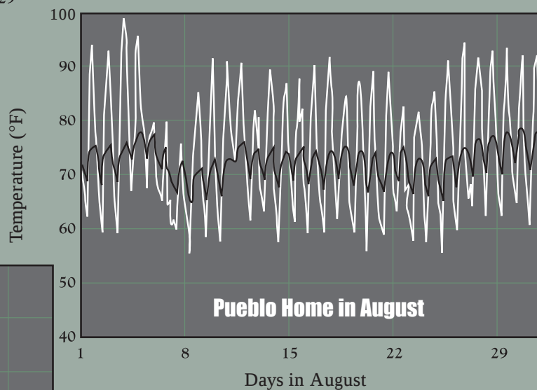
Time/temperature performance of the Pueblo home with the cooling system turned off during August.
