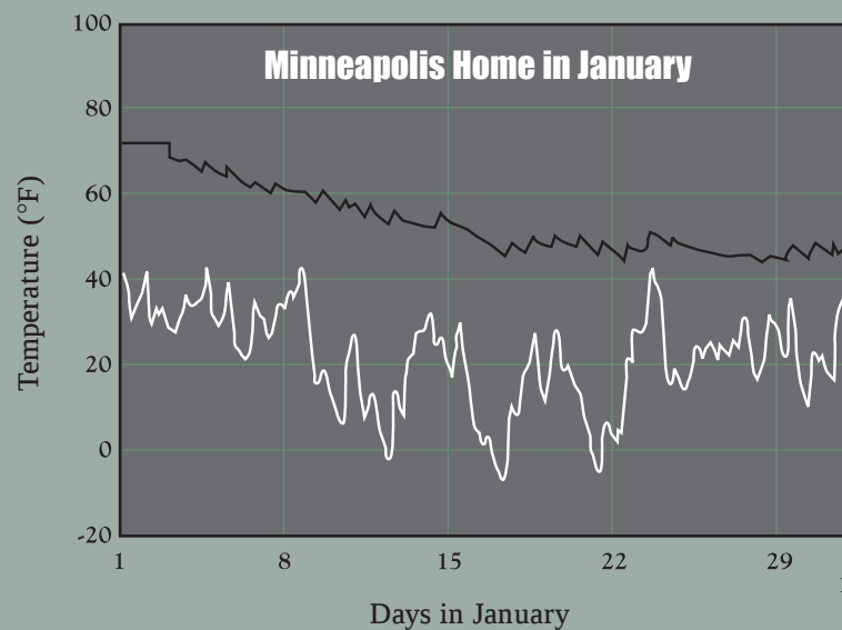
Estimated performance of the simulated house during January in Minneapolis.
