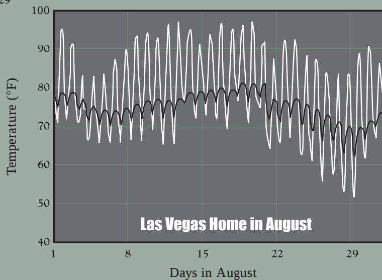
Estimated performance of the simulated house during August in Las Vegas.
