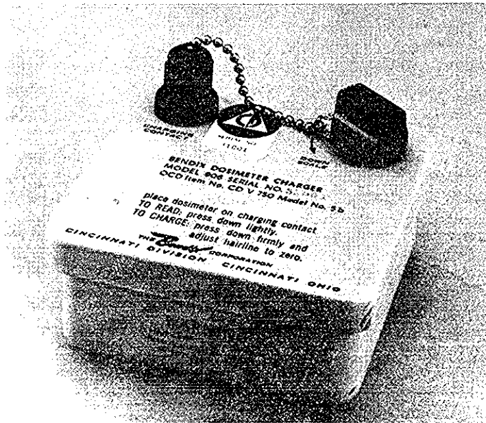
Figure 2-3. Dosimeter charger.
