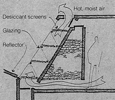
Fig. 2 Desiccant regeneration
