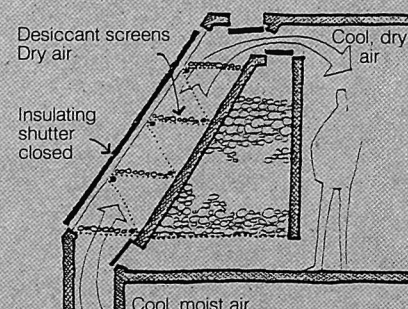
Fig. 3 Desiccation mode
