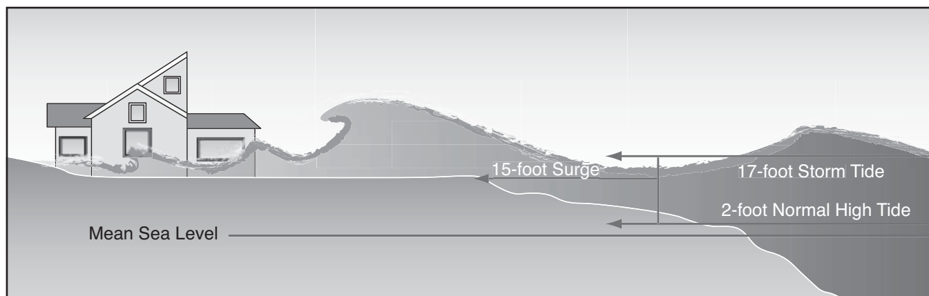
Figure I-5. Storm surge
