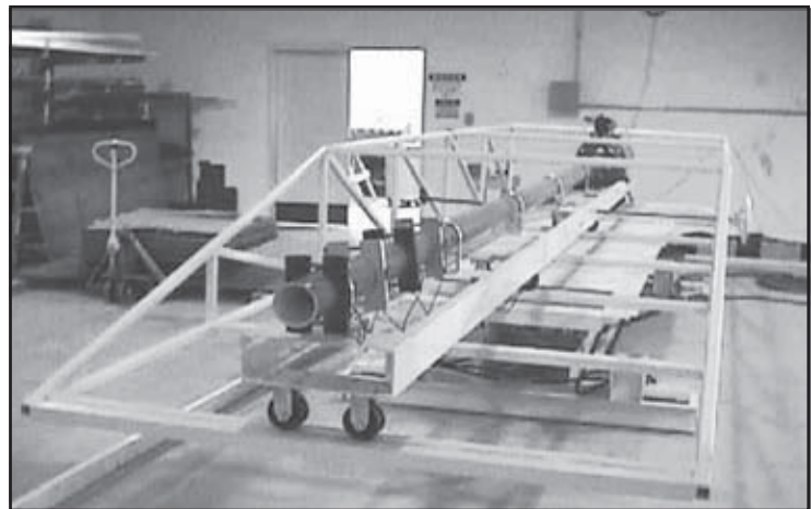
Missile (debris) launcher, Wind Engineering Research Center (WERC), Texas Tech University
