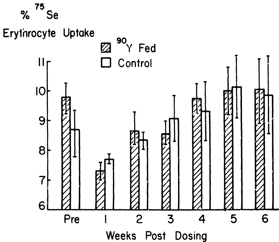
Figure 7. Effects of 90 Y Feeding on In Vitro Uptake of 75 Se by Sheep Erythrocytes.
