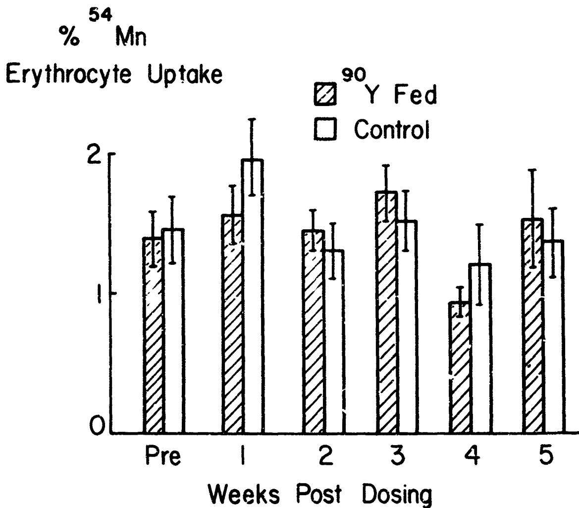
Figure 8. Effects of Feeding 90 Y on In Vitro 54 Mn Uptake by Sheep Erythrocytes.
